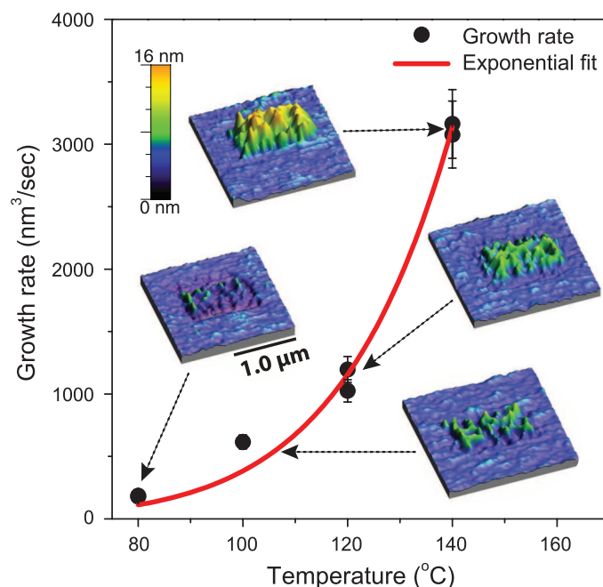
Fig. 3. Tribofilm volumetric growth rate dependence on temperature. Growth rate (mean \pm SD) versus temperature data fitted with an exponential function (Eq. 1). The 2 \mu\text{m} \times 2 \mu\text{m} topographic contact-mode AFM images shown were acquired at a nonperturbative load after generating tribofilms in the central 1.0 \mu\text{m} \times 0.5 \mu\text{m} regions at 80°, 100°, 120°, and 140°C at an initial contact pressure of ~4.4 GPa.
