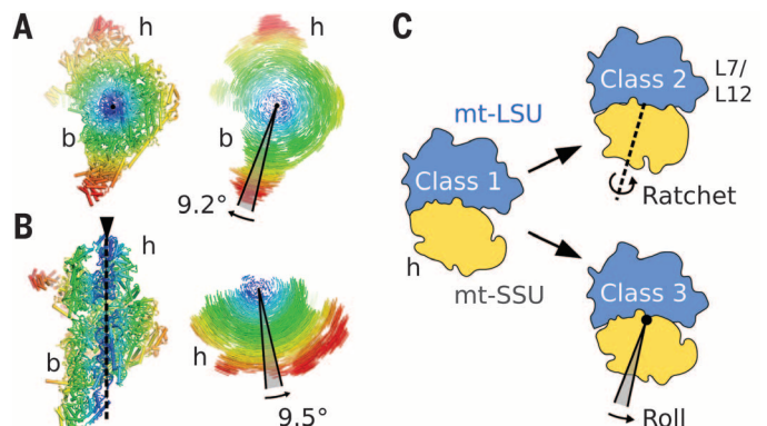
Fig. 3. Dynamics of intersubunit orientations. (A and B) Comparison of mt-SSU orientations based on common superposition of the mt-LSU. Shifts between equivalent rRNA phosphorus atoms and protein Ca atoms in the different states are color-coded (0 to 20 Å). (A) Intersubunit rotation resembling the ratchetlike mechanism common to all ribosomes. (B) Rotation of the small subunit around its long axis. (C) Schematic of mitoribosomal conformational changes.
