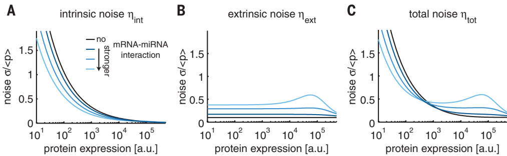
Fig. 2. Predictions of the noise model for a miRNA-regulated gene.
