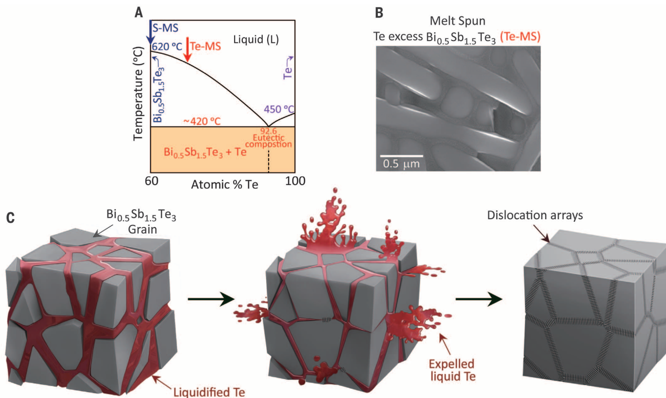
Fig. 3. Generation of dislocation arrays at grain boundaries in \text{Bi}_{0.5}\text{Sb}_{1.5}\text{Te}_3 .
