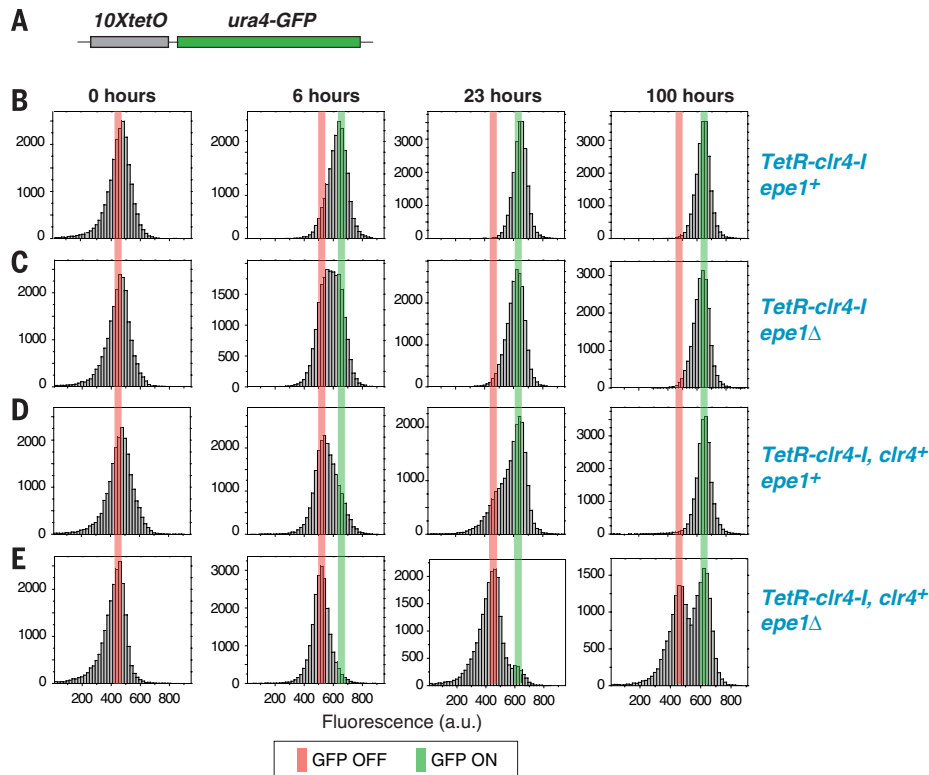
Fig. 4. Kinetics of decay of the silent state after release of TetR-Clr4-I using a GFP reporter gene reveals epigenetic maintenance in epe1 + cells. (A) Schematic diagram of the 10 XtetO - ura4-GFP locus. (B to E) FACS analysis of GFP expression in the indicated strains at 0, 6, 23, and 100 hours after tetracycline addition shows the time evolution of the distribution of GFP-OFF cells. a.u., arbitrary units. (F) Data for time points between 0 and 100 hours after addition of tetracycline were plotted to display the fraction of GFP-OFF cells as a function of time. Dose-response curve fitting was used as a guide.
