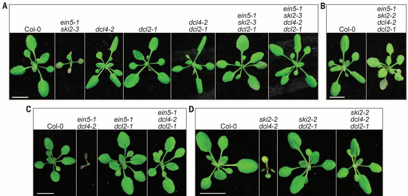
Fig. 3. Genetic interaction between the PTGS and RNA decay pathways. (A to D) Rosette morphology of 19-day-old plants was shown. No ein5-1 ski2-3 dcl4-2 plant was viable based on genotyping the segregating population derived from the ein5-1 ski2-3 hemizygote and dcl4-2 dcl2-1 cross (A). Similarly, the ein5-1 ski2-2 double mutants were not viable, and by genotyping the F_2 and F_3 plants propagated from the ein5-1 ski2-2 hemizygote and dcl4-2 dcl2-1 cross, no ein5-1 ski2-2 dcl2-1 or ein5-1 ski2-2 dcl4-2 triple mutants were viable (B). Scale bars, 1 cm.
