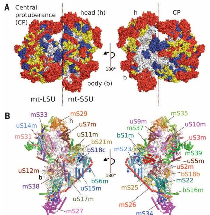
Fig. 2. Overview of the human mitoribosome. (A) Proteins conserved with bacteria (blue), extensions of homologous proteins (yellow), and mitochondria-specific proteins (red). rRNA is shown in gray. (B) Location of proteins in the human mt-SSU.
