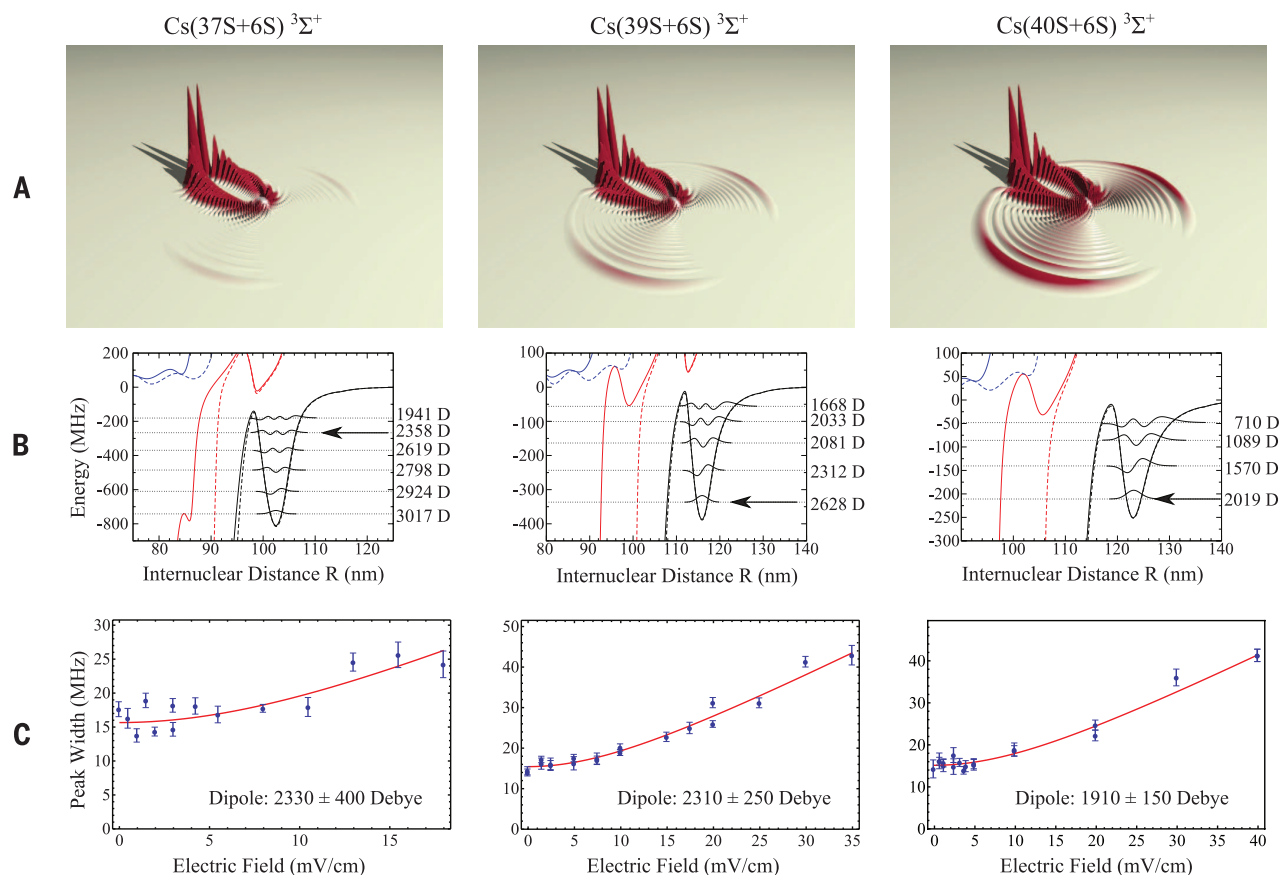
Fig. 1. Trilobite states in Cs molecules. (A) The electron probability distribution |\Psi(R_e; \mathbf{r})|^2 (Eq. 1) for the molecular states red-detuned from \text{Cs}(n = 37S, 39S, and 40S) Rydberg lines, each marked in (B) with an arrow, in cylindrical coordinates. The Rydberg ion is located near the center of each plot, and the Rydberg electron is localized near the location of the ground-state perturber. The distributions are shown at the equilibrium separations at R_e = 102.4, 115.9, and 123.0 \text{ nm} for the corresponding BO PECs, given in (B). (B) The BO PECs (black, red, and blue curves) correlate asymptotically to the nS + 6S,
